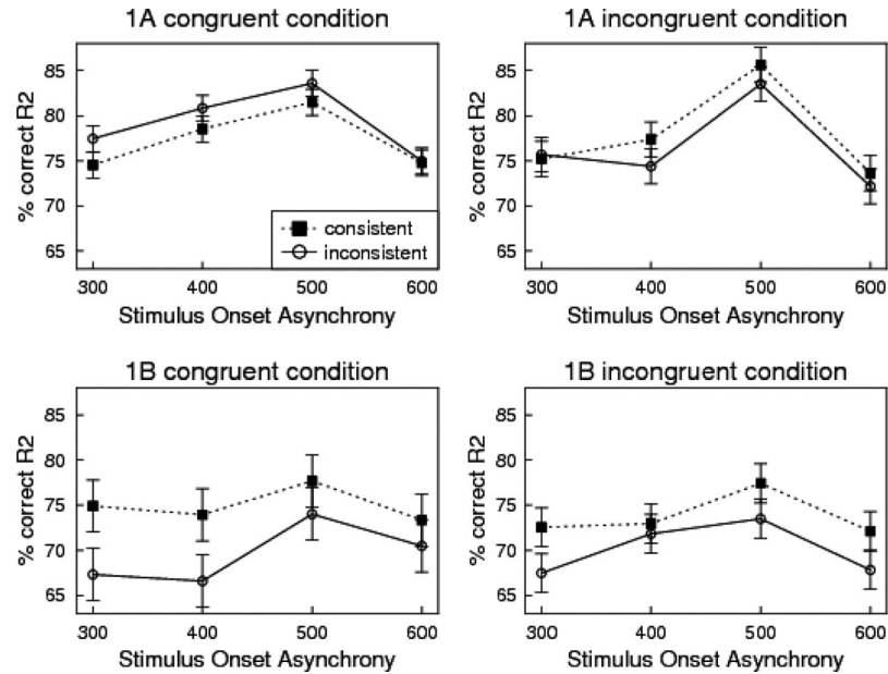
Figure 3. Mean R2 accuracy in Experiment 1 for each condition in relative to SOA. Filled squares represent consistent trials, and empty circles represent inconsistent trials. The four panels represent groups of participants that differed in the R1-S1 mapping (congruent vs. incongruent) and in experiment (Experiment 1A vs. Experiment 1B). Confidence intervals have been calculate according to Loftus and Masson (1994; Masson & Loftus, 2003) for within-subjects comparisons of consistency, collapsed over SOA, but separately for each congruency group.
