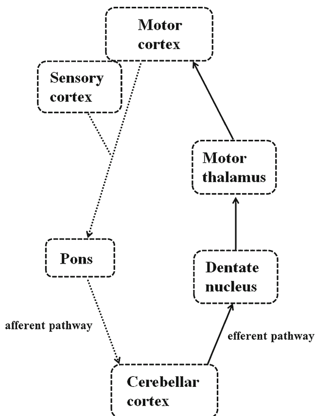
Fig. 1 Simplified scheme of the fronto-pontine-cerebello-thalamo-cortical loop. Solid lines indicate the cerebellar efferent pathways and dotted lines the cerebellar afferent pathways (from Groiss and Ugawa [10], with permission)
